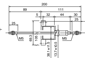
CMS5D20-1PF
