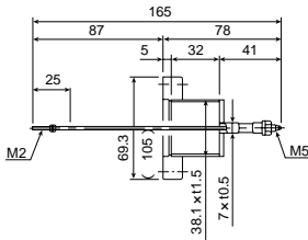
CMS2D09-1PF
