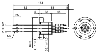
CMS2D09-8PF 6
