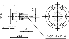
CMS1DTMC-2PFM 7
