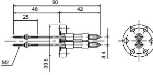
CMS2D09-2PFM 6
