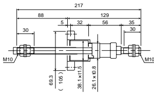
CMS10D20-1PF
