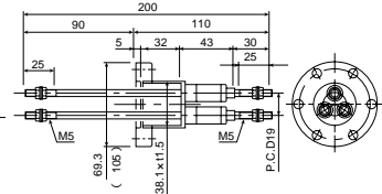
CMS5D20-3PF
