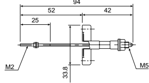
CMS2D09-1PFM
