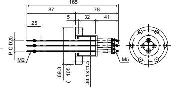
CMS2D09-4PF
